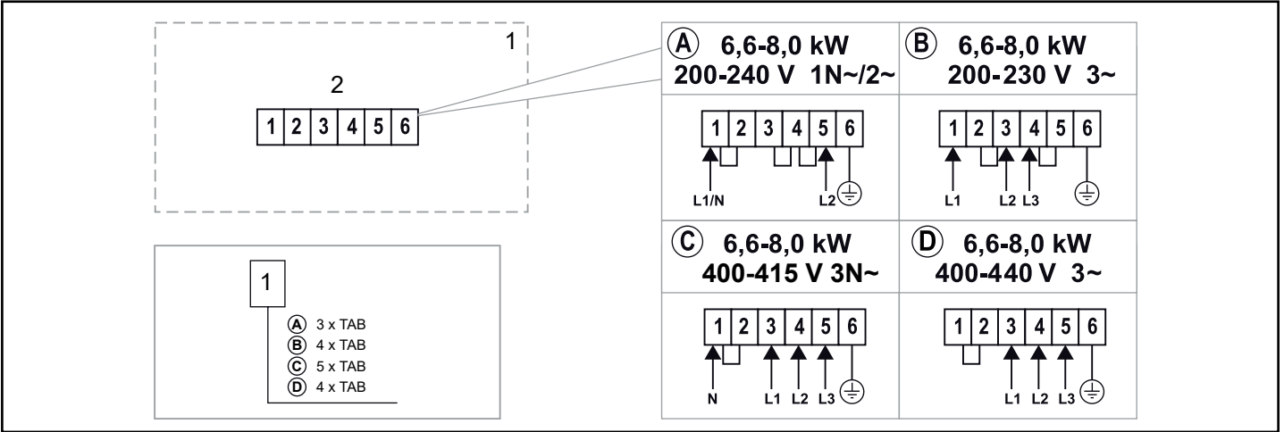
Figure 12: Wiring diagram 1. Heater 2. Terminal for connection of electrical cable
